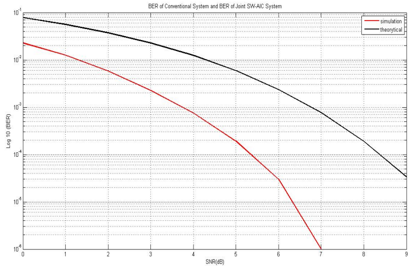
Figure 5.0 BER
