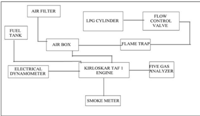
Figure 3: Experimental layout
