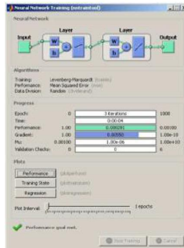
Fig2: Neural network training tool [1]
