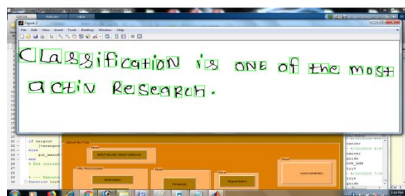
Fig6: Character extraction
