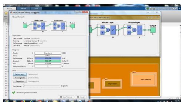
Fig7: Train Network
