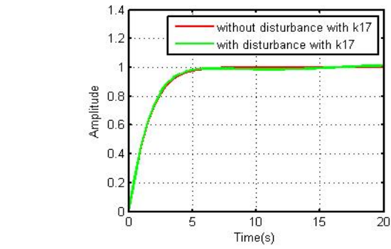
Figure 16: Step response of the controlled plant using k17 with and without disturbance
