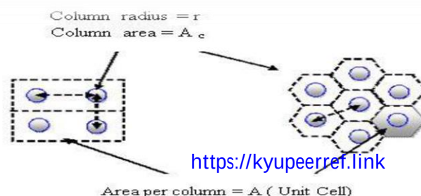
Figure: 1 Plan of stone column, Square pattern and Triangular pattern (Cabe,2007)
