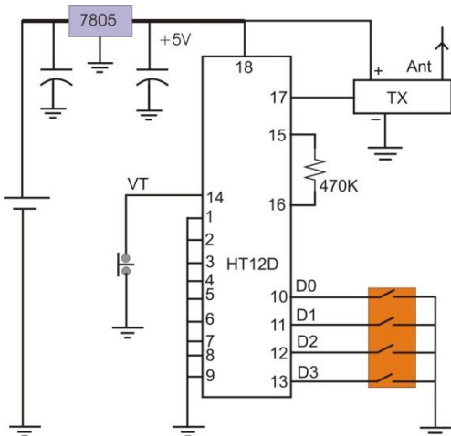
FIG 5: Circuit Diagram of Transmitter
