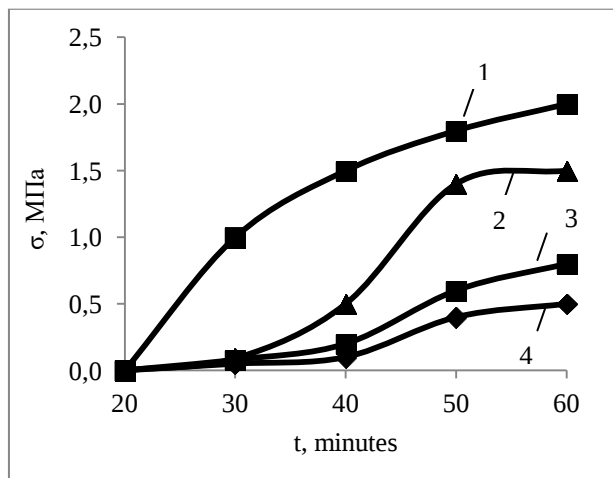
Fig. 1. Residual stresses of epoxy binders ( \sigma ) vs curing time ( t ) at T= 80\text{ }^{\circ}\text{C} : 1 – without nanofiller; 2 – 0,5 wt. p. of CNTs; 3- 0,5 wt. p. of OM; 4 – 0,5 wt. p. of ANT
