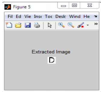
Fig.7. Extracted Image
